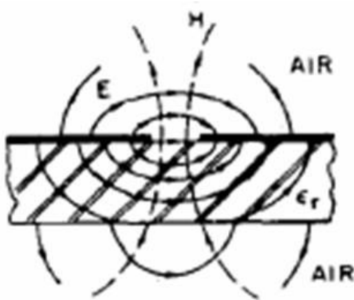
Fig. 3 Field Lines for Slot line mode
