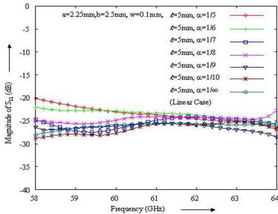
Fig. 8 Characteristics of NRD Guide to NRD-Slot line Transition
