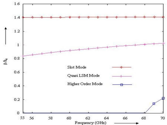
Fig. 5 Dispersion Characteristics of NRD Guide
