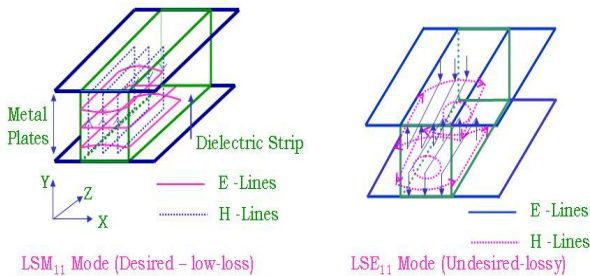
Fig.2. Propagating modes in NRD Guide
