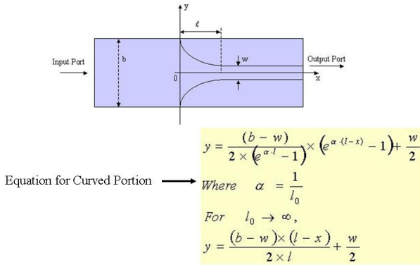
Fig. 7 Transition from NRD Guide to Integrated NRD-Slot Line
