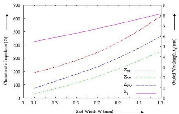
Fig. 6 Variation of Guide wavelength and Characteristic Impedance with slot width
