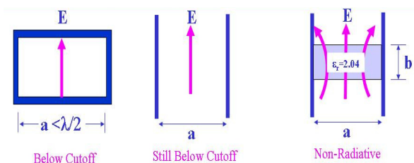
Fig. 1 Concept of NRD Guide
