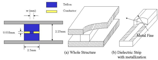
Fig. 4 Integration of NRD Guide and Slot Line
