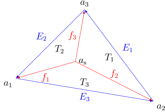
Figure 1: Triangle T with splitting
