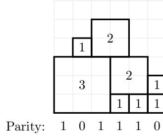
Figure 7: Example for the parity change by placing squares.
