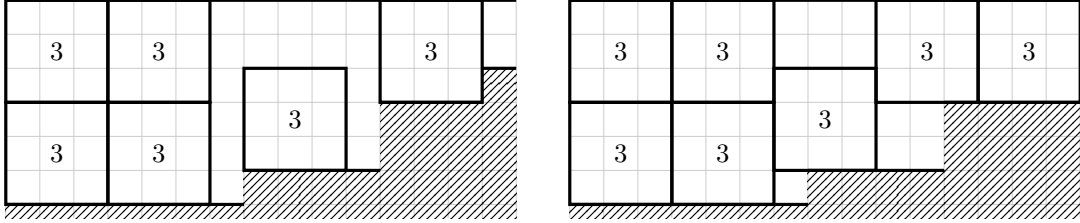
Figure 4: Example for different flow defects. In the left picture we have D_3(f) = 2 and in the right D_3(f) = 3 . A maximal placement of squares of size 3 is shown. In the right picture we can place one square more, due to the overhang that is now possible.
